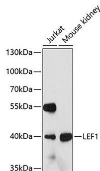
Fig. 1. Western blot analysis of extracts of various cell lines, using LEF1 antibody at 1:3000 dilution. Secondary antibody: HRP-labeled Goat Anti-Rabbit IgG(H+L) (A0208) at 1:1000 dilution. Lysates/proteins: 25µg per lane. Blocking buffer: QuickBlock™ Blocking Buffer (P0231). Detection: BeyoECL Star (P0018A). Exposure time: 1s.
